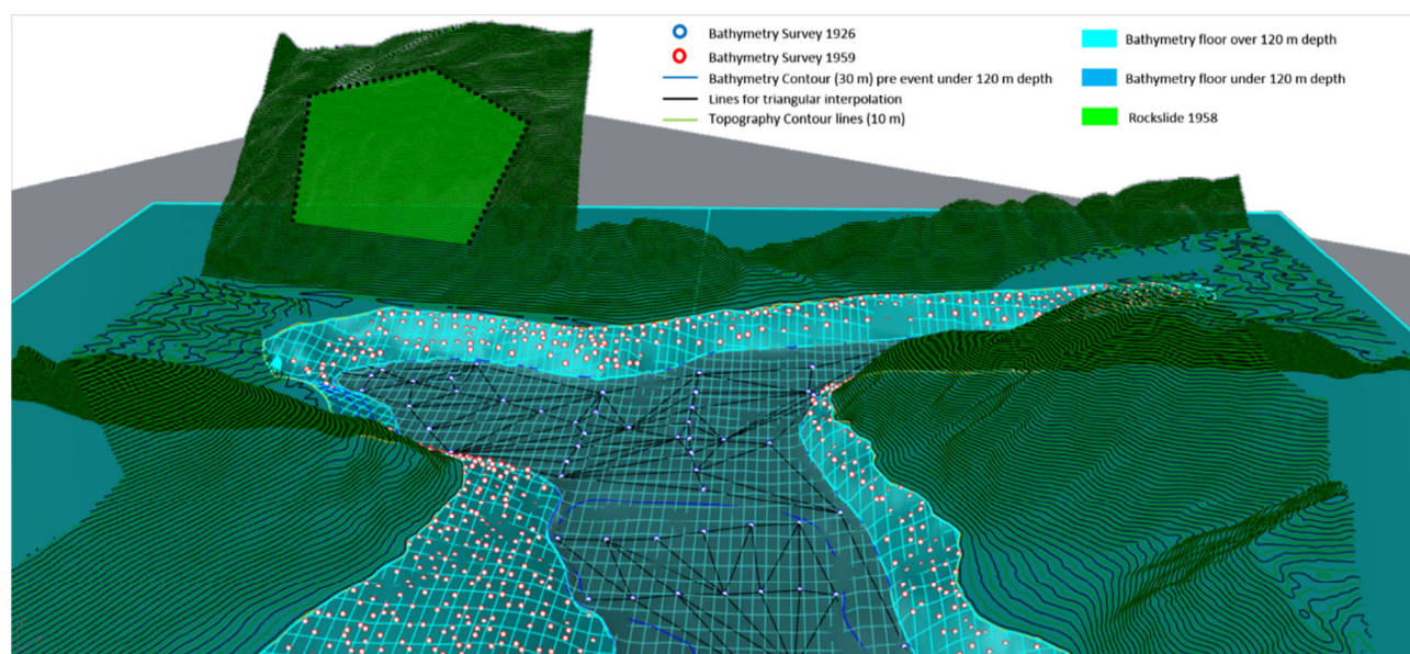
Fig.2: Reconstruction of the Lituya Bay bathymetry 1958 based on data from U.S. Coast and Geodesic Survey: Survey id: H04608, 1926 and Survey id: H08492, 1959. DTM available from DGGS Elevation Portal of Alaska.
